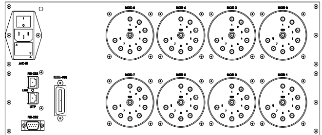
CXM/64 with IEEE488, RS232 & LAN Control
