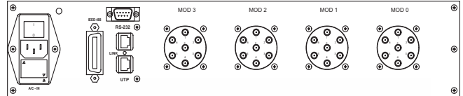
CXM/32 with IEEE488, RS232 and LAN Control
