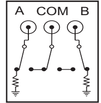
Fig. 4 CXM/2x1-T Terminated Switch
