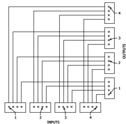
Fig. 1 4x4 Matrix Using Eight CXM/4x1 Switches
