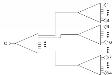
Fig. 2 64x1 Multiplexer using nine CXM/8x1 Switches
