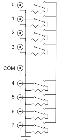
Fig. 5 CXM/8x1-T Terminated Switch
