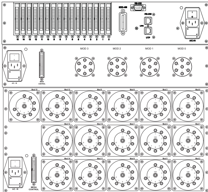
MESA Control Mainframe with CXM/32-E and CXM/128-E Expansion Chassis
